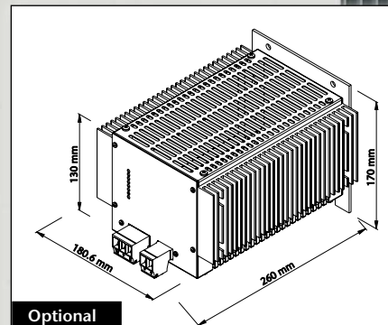
Optional Wall mount approx. 6.0 kg
