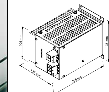
Optional Chassis mount approx. 2.1 kg
