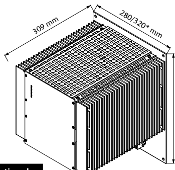
Optional Wall mount approx. 19 kg/ *) 22 kg *) applicable to models >= 150 A input or output current
