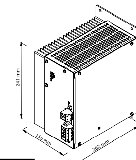
Optional Chassis mount approx. 7.5 kg (available for currents up to 60Amps)
