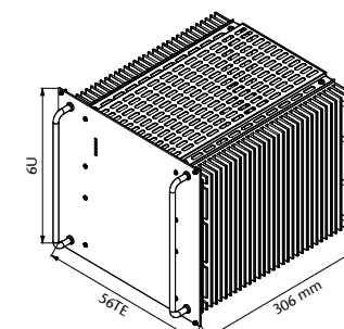
Standard Eurocassette (pluggable module for 19" sub-rack)
