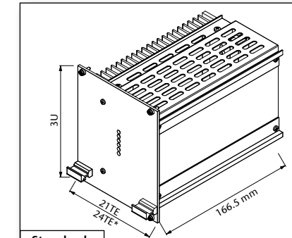
Standard Eurocassette (pluggable module for 19" sub-rack) *) applicable to 5 V output models approx. 1.7 kg
