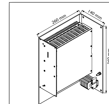
Optional Wall mount approx. 8.0 kg
