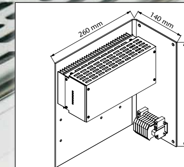
Optional Wall mount approx. 5.0 kg
