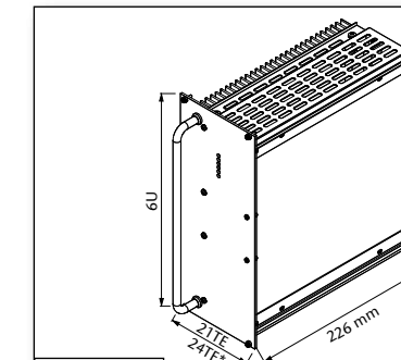
Standard Eurocassette (pluggable module for 19" sub-rack) approx. 5.0 kg *) applicable to 5 V output models
