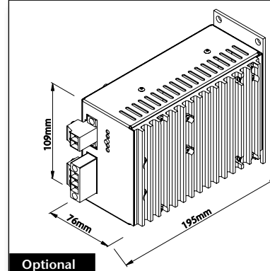
Optional Chassis mount approx. 1.05 kg
