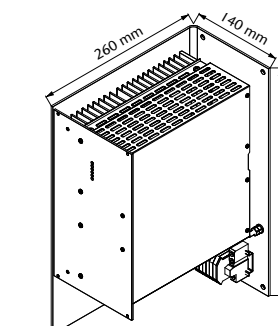
Optional Wall mount approx. 9.5 kg
