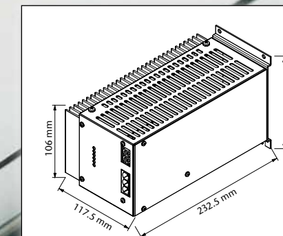
Optional Chassis mount approx. 3.0 kg
