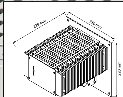
Optional Wall mount approx. 6.0 kg
