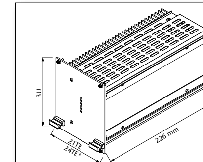
Standard Eurocassette (pluggable module for 19" sub-rack) approx. 2.5 kg *) applicable to 5 V output models
