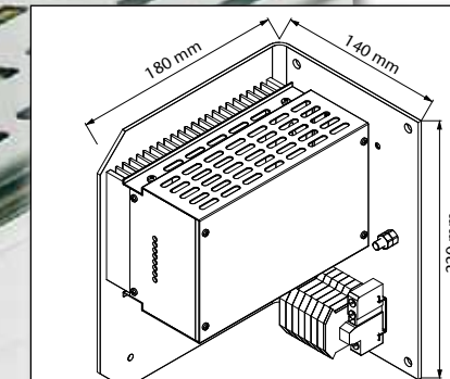
Optional Wall mount approx. 3.2 kg
