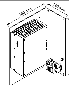
Optional Wall mount approx. 6.3 kg
