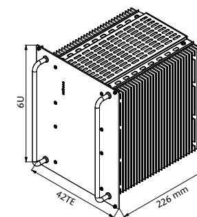
Standard Eurocassette (pluggable module for 19" sub-rack) approx. 10.0 kg
