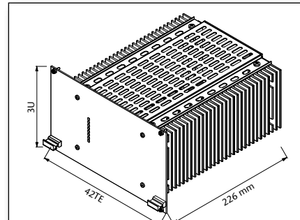
Standard Eurocassette (pluggable module for 19" sub-rack) approx. 4.0 kg
