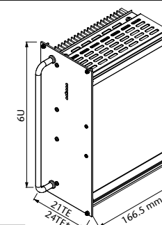
Standard Eurocassette (pluggable module for 19" sub-rack) approx. 3.3 kg (*) applicable to 5 V output models
