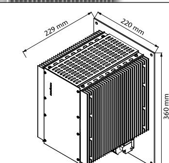
Optional Wall mount approx. 12.5 kg
